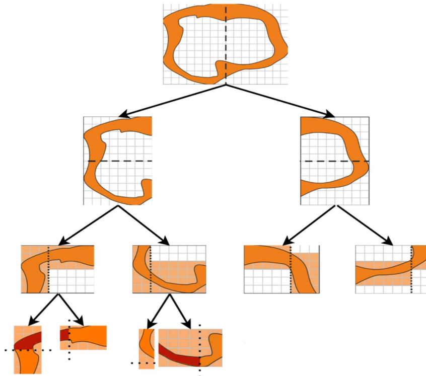
Figure 18: Recursive splitting of the cluster; dashed lines: C-splitting, dotted lines: L-splitting, wide-dotted lines: information-based splitting
