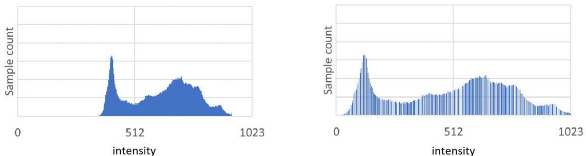
Figure 20: Histogram of a chroma component of a source view: before (left) and after (right) dynamic range scaling
