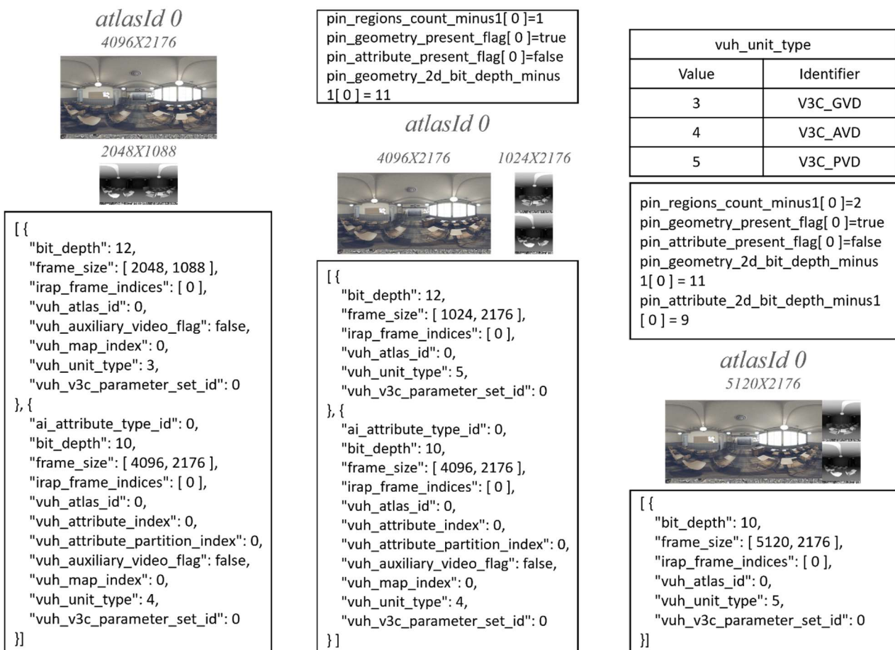
Figure 28: Geometry packing for MIV anchor – ClassroomVideo sequence at frame 0: MIV anchor (left), geometry packing (center), geometry packing + attribute bitstreams merging (right)
