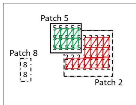
Figure 40: Creating a mesh from an atlas. Triangles between pixels from Patch 5 and 2 are omitted. Note that Patch 8 is not drawn because no triangle can be formed. Unused pixels are skipped too
