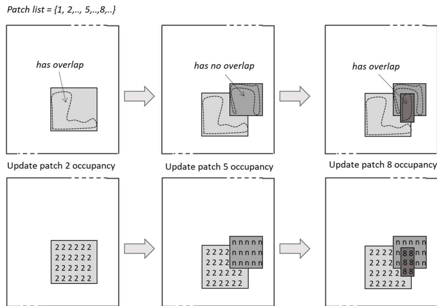
Figure 38. Occupancy map update in an ordered manner with patch culling
