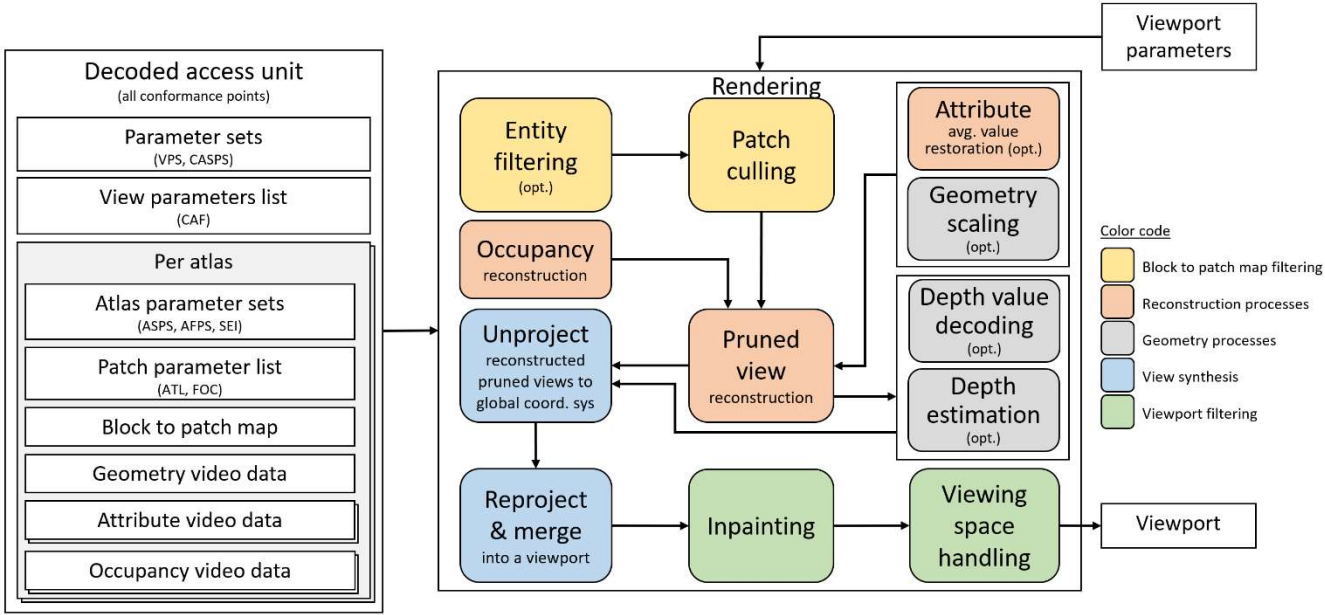
Figure 37: Process flow for the TMIV renderer
