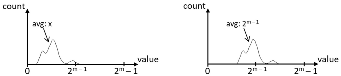
Figure 21: Histogram of an attribute component of a patch: before (left) and after (right) average value modification
