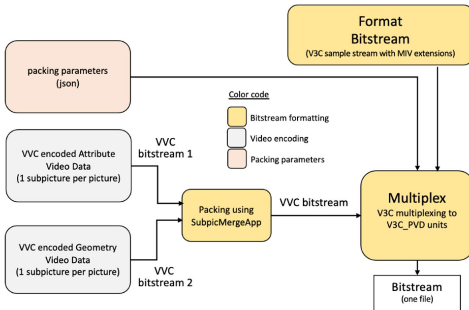
Figure 29: Encoding of texture and geometry components into one packed video sub-bitstream
