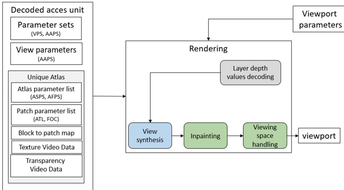
Figure 45: Process flow for TMIV MPI renderer
