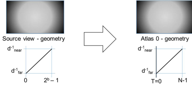
Figure 24: When the source material (with b bits per sample) has only valid geometry values, the geometry coder only performs u(b) to u(m) or u(m - 1) scaling and the geometry threshold is set to zero to signal full occupancy; N = 2^m if the geometry has a good quality (§4.2.5) and 2^{m-1} otherwise
