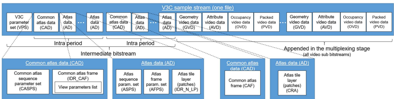
Figure 36: V3C sample stream with MIV extensions
