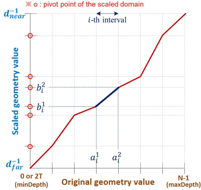
Figure 26: An example of piecewise linear scaling (for 7 intervals)
