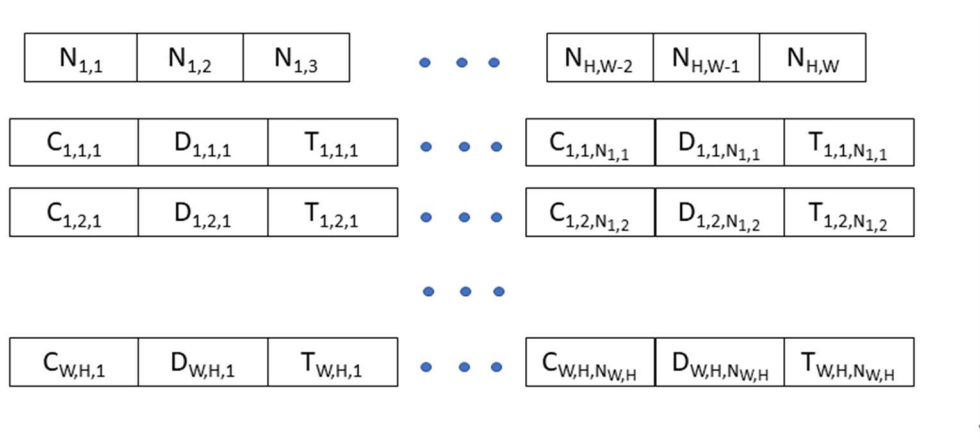
Figure 34: MPI packed compressed storage (PCS) layout.
