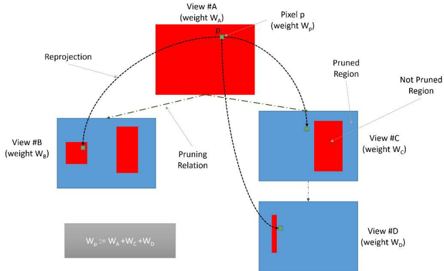
Figure 41: graph-based pruning: weight recovery procedure
