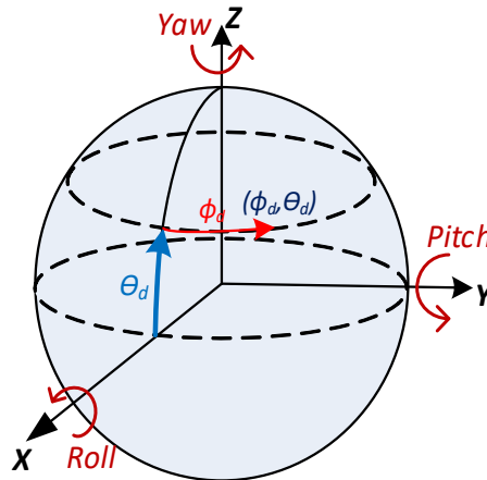
Figure 46: OMAF coordinate system illustrating the directions of positional and rotational units
