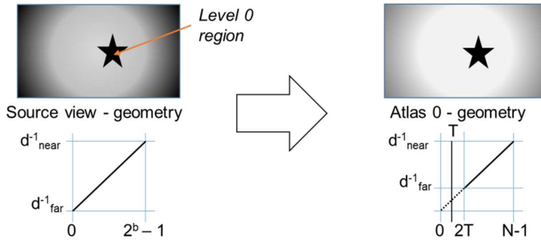
Figure 25: When the source material (with b bits per sample) has invalid geometry values, the geometry coder not only performs u(b) to u(m) or u(m - 1) scaling, but it also sets the geometry threshold to a configured value ( T ) and the normalized disparity range is modified such that value 2T corresponds to the far geometry; N = 2^m if the geometry has a good quality (§4.2.5) and 2^{m-1} otherwise
