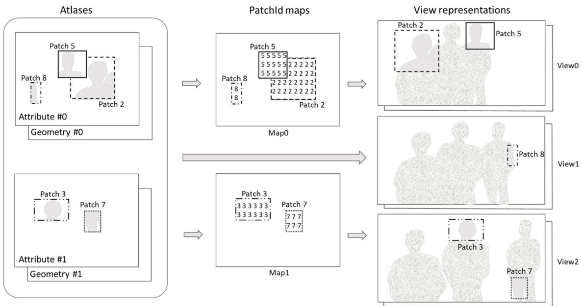
Figure 39: Pruned view reconstruction
