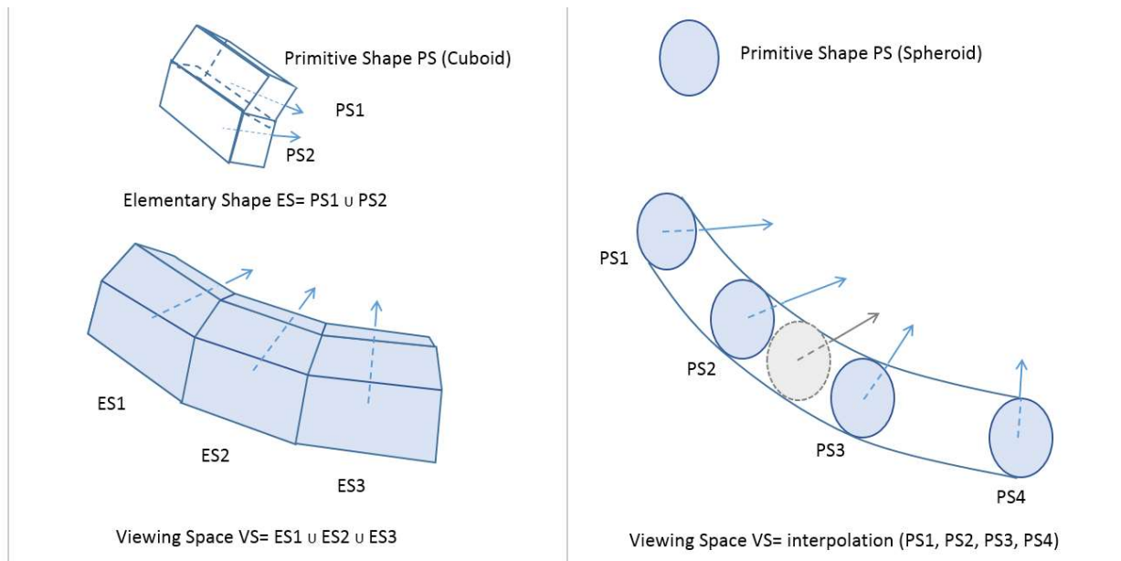
Figure 44: Illustration of VS creation with additive CSG (left) and interpolation (right)
