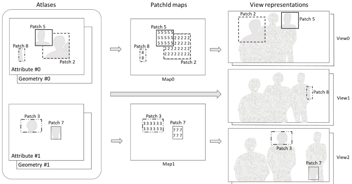
Figure 40: Pruned view reconstruction
