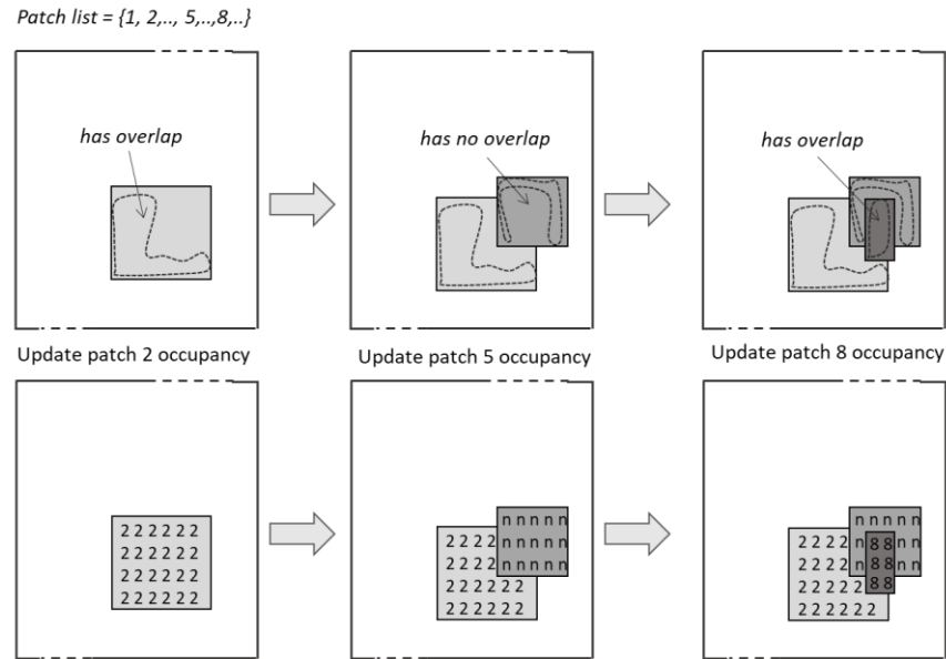
Figure 39. Occupancy map update in an ordered manner with patch culling
