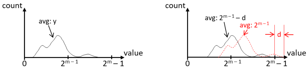
Figure 23: Histogram of an attribute component of a patch: before (left) and after (right) average value modification (overflow avoiding)
