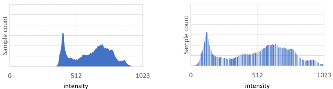
Figure 21: Histogram of a chroma component of a source view: before (left) and after (right) dynamic range scaling
