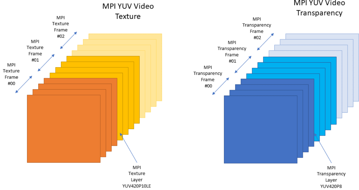
Figure 34: MPI raw storage diagram. In this simplified example, the MPI content is made of 4 layers (sorted from far to close) and 3 concatenated temporal frames
