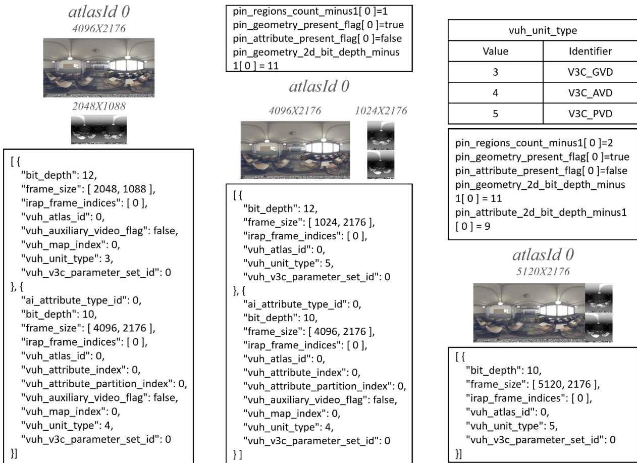
Figure 29: Geometry packing for MIV anchor – ClassroomVideo sequence at frame 0: MIV anchor (left), geometry packing (center), geometry packing + attribute bitstreams merging (right)
