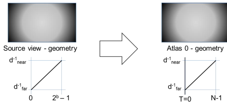
Figure 25: When the source material (with b bits per sample) has only valid geometry values, the geometry coder only performs u(b) to u(m) or u(m - 1) scaling and the geometry threshold is set to zero to signal full occupancy; N = 2^m if the geometry has a good quality (§4.2.5) and 2^{m-1} otherwise
