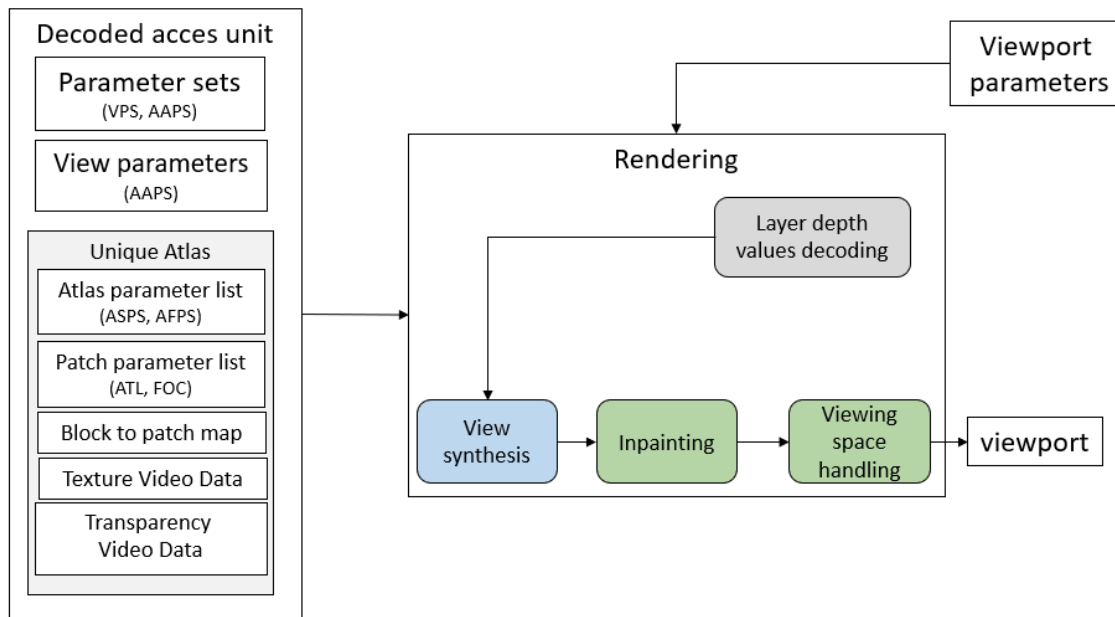
Figure 46: Process flow for TMIV MPI renderer
