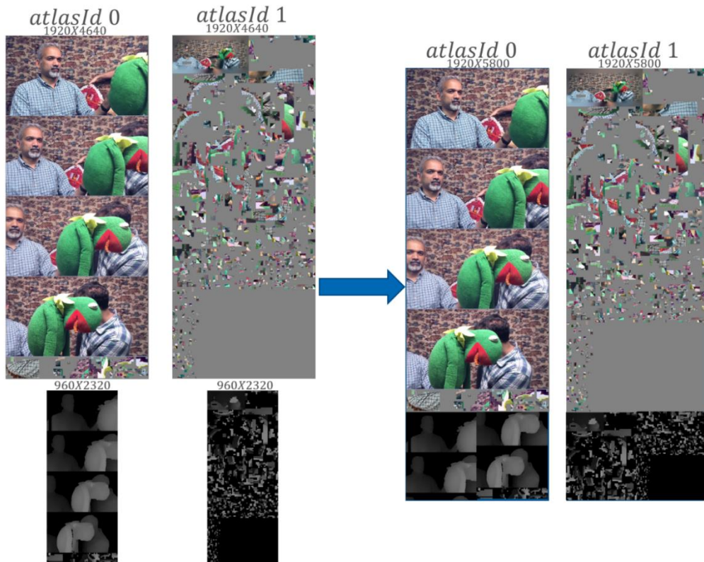
Figure 28: Frame packing for MIV anchor – Frog sequence at frame 0, featuring 3 regions
