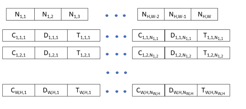
Figure 35: MPI packed compressed storage (PCS) layout.
