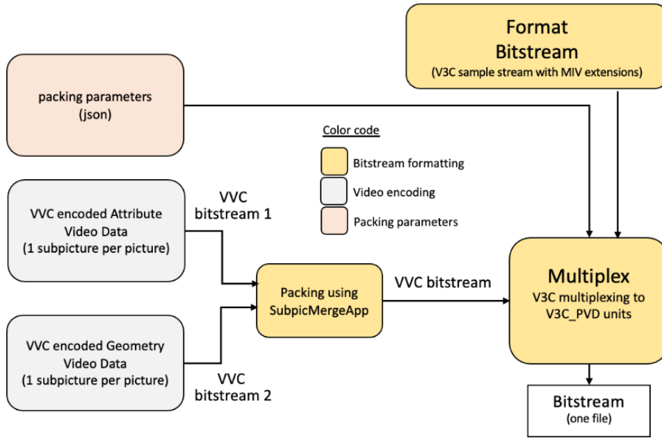
Figure 30: Encoding of texture and geometry components into one packed video sub-bitstream
