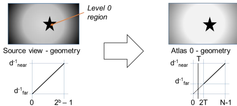
Figure 26: When the source material (with b bits per sample) has invalid geometry values, the geometry coder not only performs u(b) to u(m) or u(m - 1) scaling, but it also sets the geometry threshold to a configured value ( T ) and the normalized disparity range is modified such that value 2T corresponds to the far geometry; N = 2^m if the geometry has a good quality (§4.2.5) and 2^{m-1} otherwise
