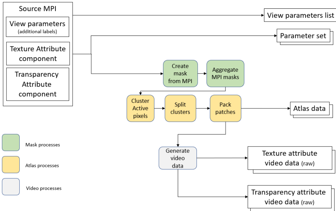
Figure 36: Top-level diagram of the TMIV MPI encoder
