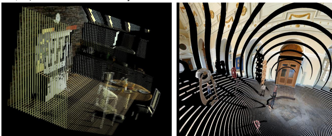
Figure 32: Texture MPI layers of different projections; perspective Kitchen (left) and equirectangular Museum (right)
