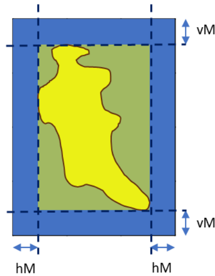
Figure 19: Positioning of cluster (yellow) within a patch (blue); hM and vM are horizontal and vertical margins of the patch, transmitted within metadata.
