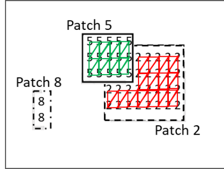
Figure 41: Creating a mesh from an atlas. Triangles between pixels from Patch 5 and 2 are omitted. Note that Patch 8 is not drawn because no triangle can be formed. Unused pixels are skipped too
