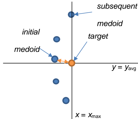
Figure 10: Initial basic view selection
