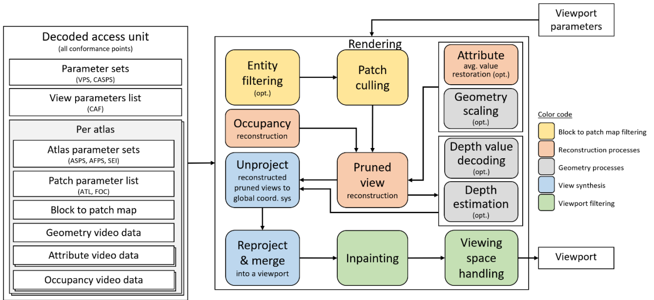
Figure 39: Process flow for the TMIV renderer
