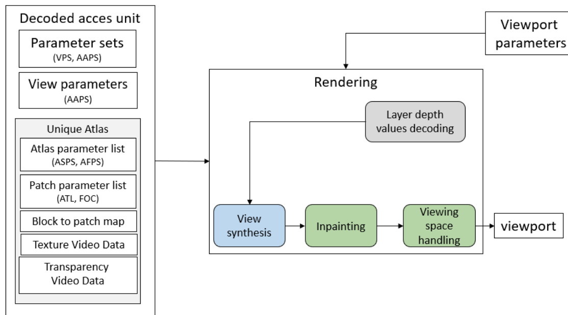
Figure 47: Process flow for TMIV MPI renderer
