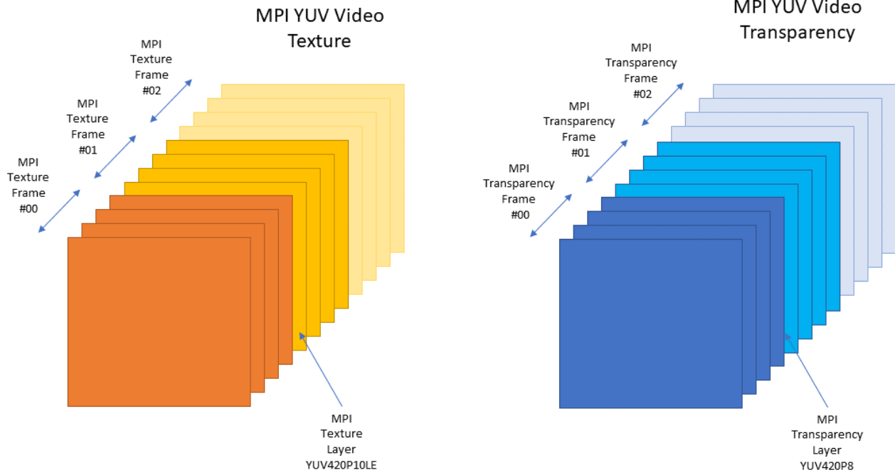
Figure 35: MPI raw storage diagram. In this simplified example, the MPI content is made of 4 layers (sorted from far to close) and 3 concatenated temporal frames
