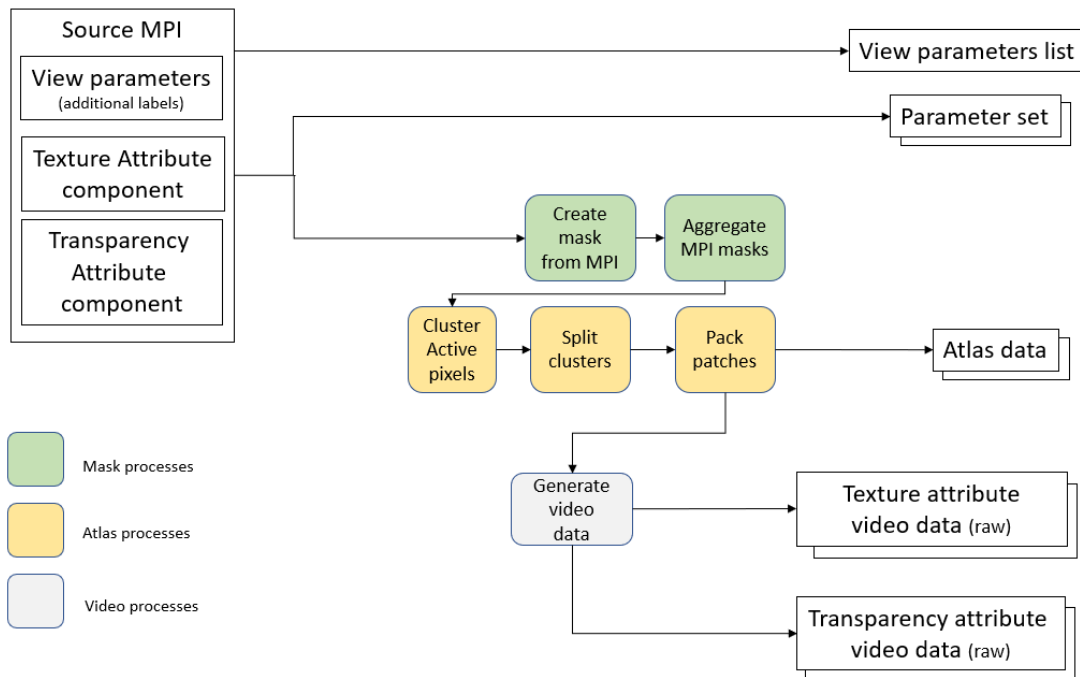
Figure 37: Top-level diagram of the TMIV MPI encoder
