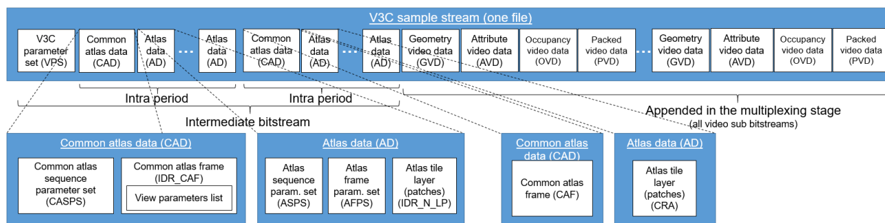
Figure 38: V3C sample stream with MIV extensions
