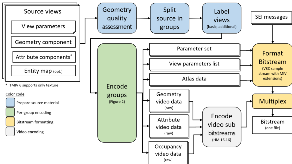
Figure 1: Top-level diagram of the TMIV group-based encoder
