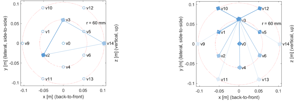
Figure 8: Repulsion of medoids v_2 and v_3 and v_{14} (left) and attraction of medoid v_3 to non-medoids (right)
