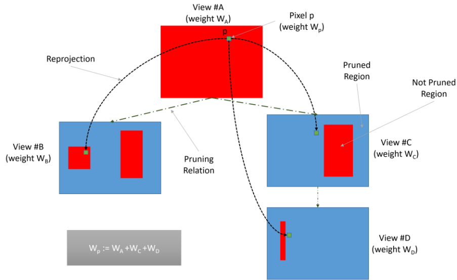
Figure 26: graph-based pruning: weight recovery procedure
