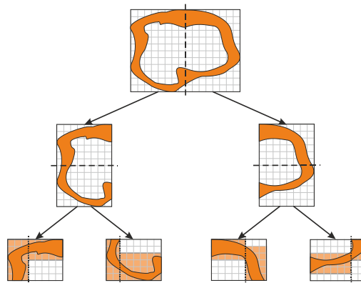
Figure 16: Recursive splitting of the cluster; dashed lines: C-splitting, dotted lines: L-splitting
