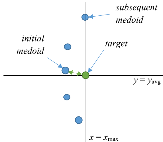
Figure 9: Initial basic view selection
