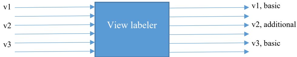
Figure 6: View selection behavior of the view labeler when outputAdditionalViews is true
