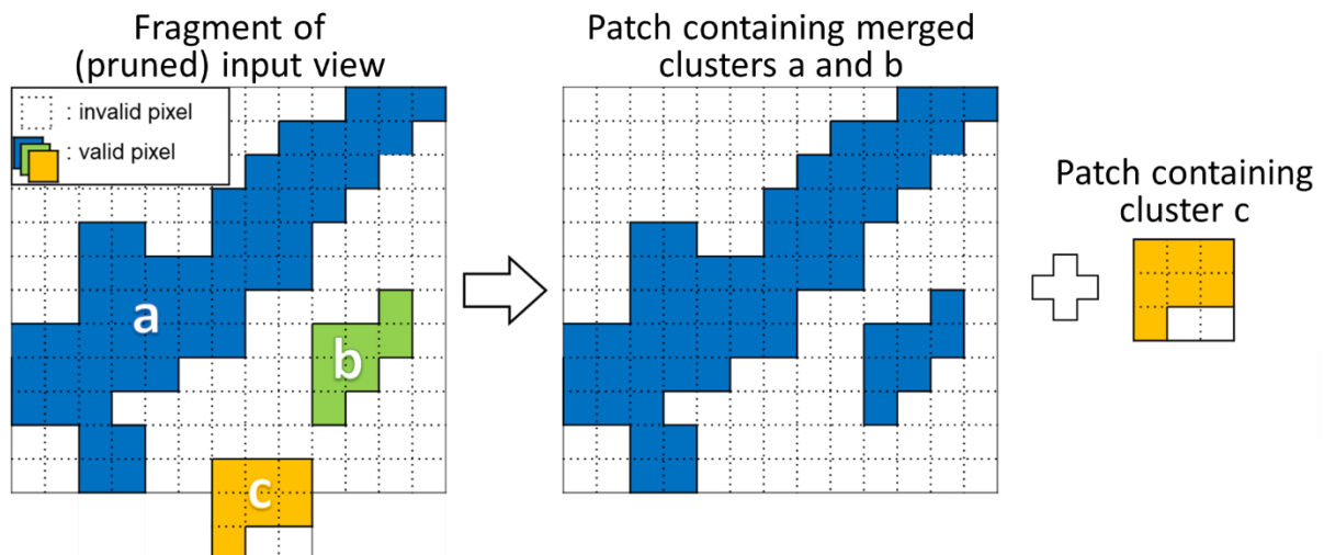
Figure 15: An example of cluster merging
