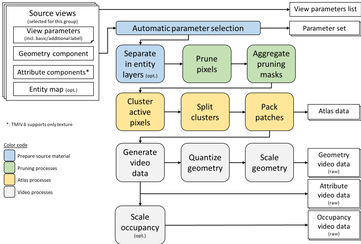
Figure 2: Top-level diagram of the TMIV single-group encoder
