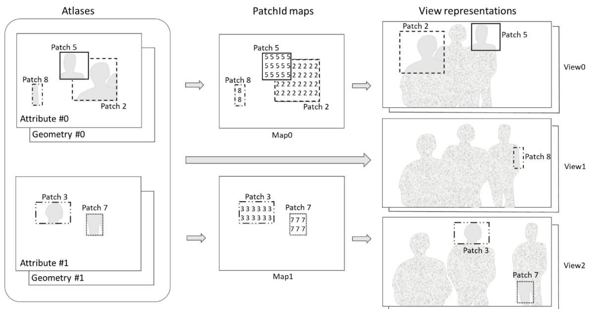
Figure 24: Pruned view reconstruction
